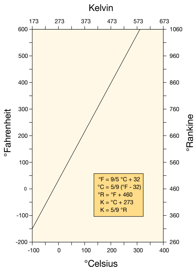
Fig. 7.1 Temperature conversion
