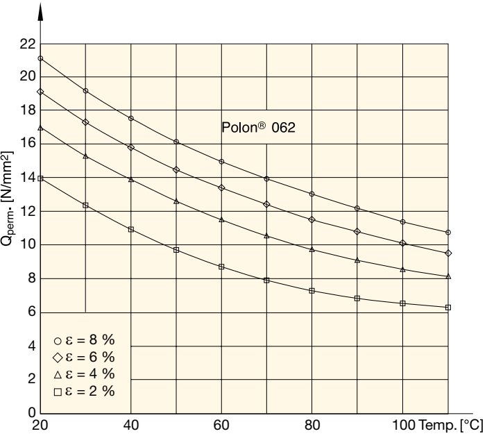
Permissible specific load Q perm. in relation to temperature t and the respective permanent set ε for the compounds Polon® 062:
