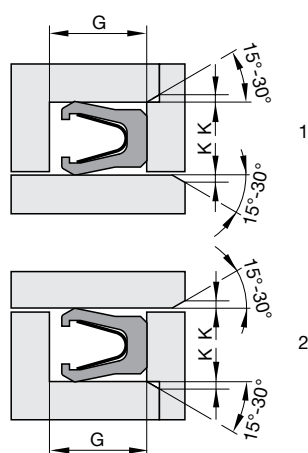
Fig. 3.33 Two-piece groove "lips first" installation; 1) rod, 2) piston
