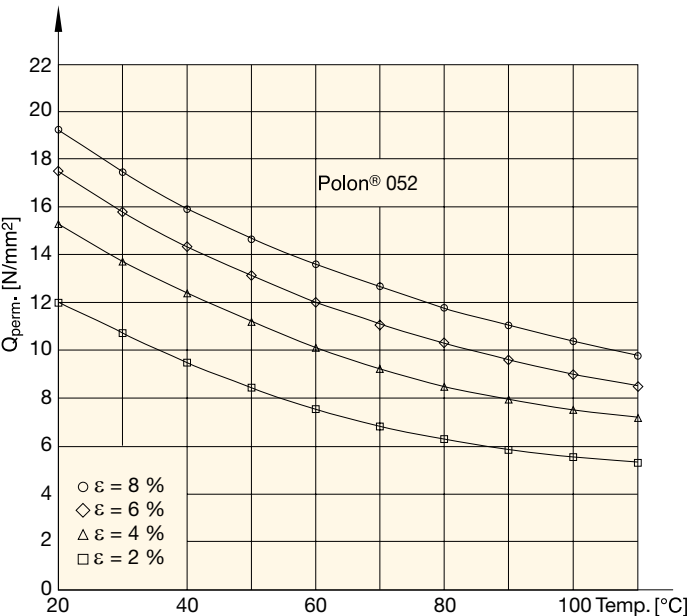
Permissible specific load Q perm. in relation to temperature t and the respective permanent set ε for the compounds Polon® 052:
