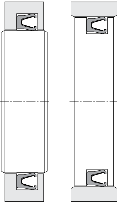
Fig. 3.38 Closed-groove configurations in rod and piston mode
